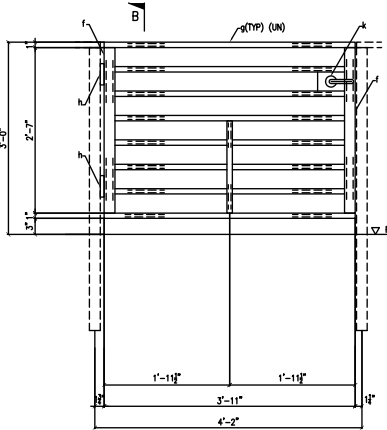
ONE - DOOR - 6D (REF./L-3)
