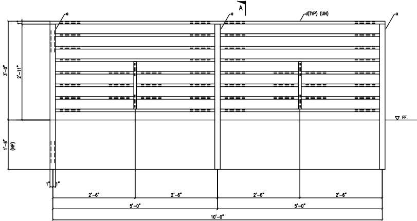
ONE - FENCE - 6C (REF./L-3)
