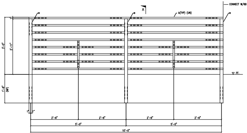
ONE - FENCE - 6A (REF./L-3)
