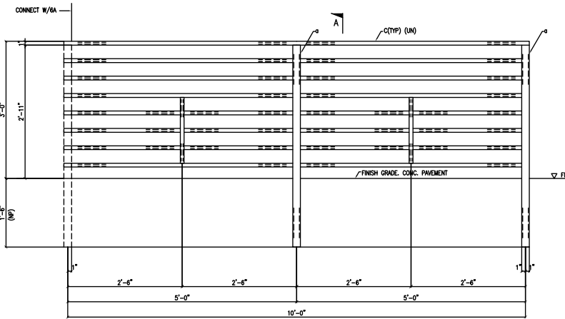
ONE - FENCE - 6B (REF./L-3)
